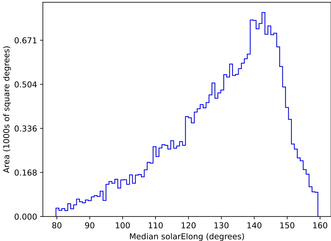
too_elab_r64_d3_ugrizy_v3.4_10yrs All sky g band: Median solarElong
