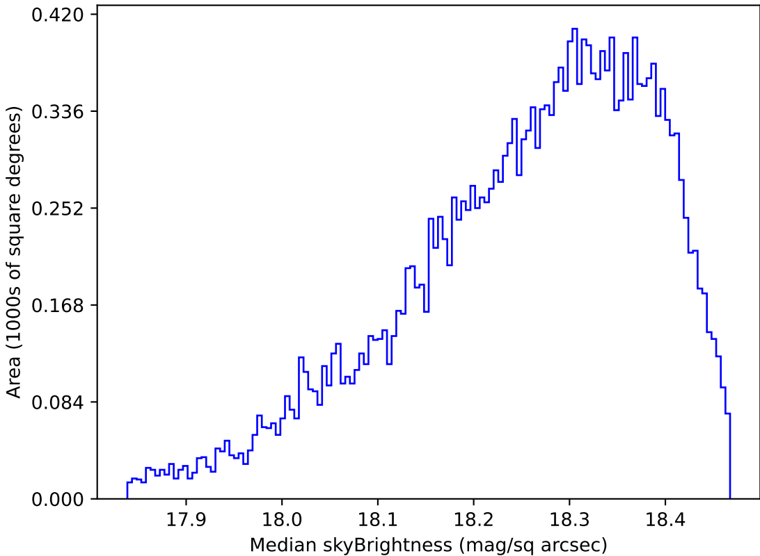
too_elab_r64_d3_ugrizy_v3.4_10yrs Yr 1 y band: Median skyBrightness
