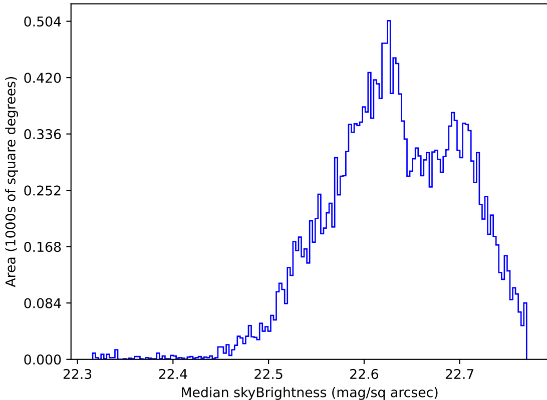
too_elab_r64_d3_ugrizy_v3.4_10yrs Yr 1 u band: Median skyBrightness
