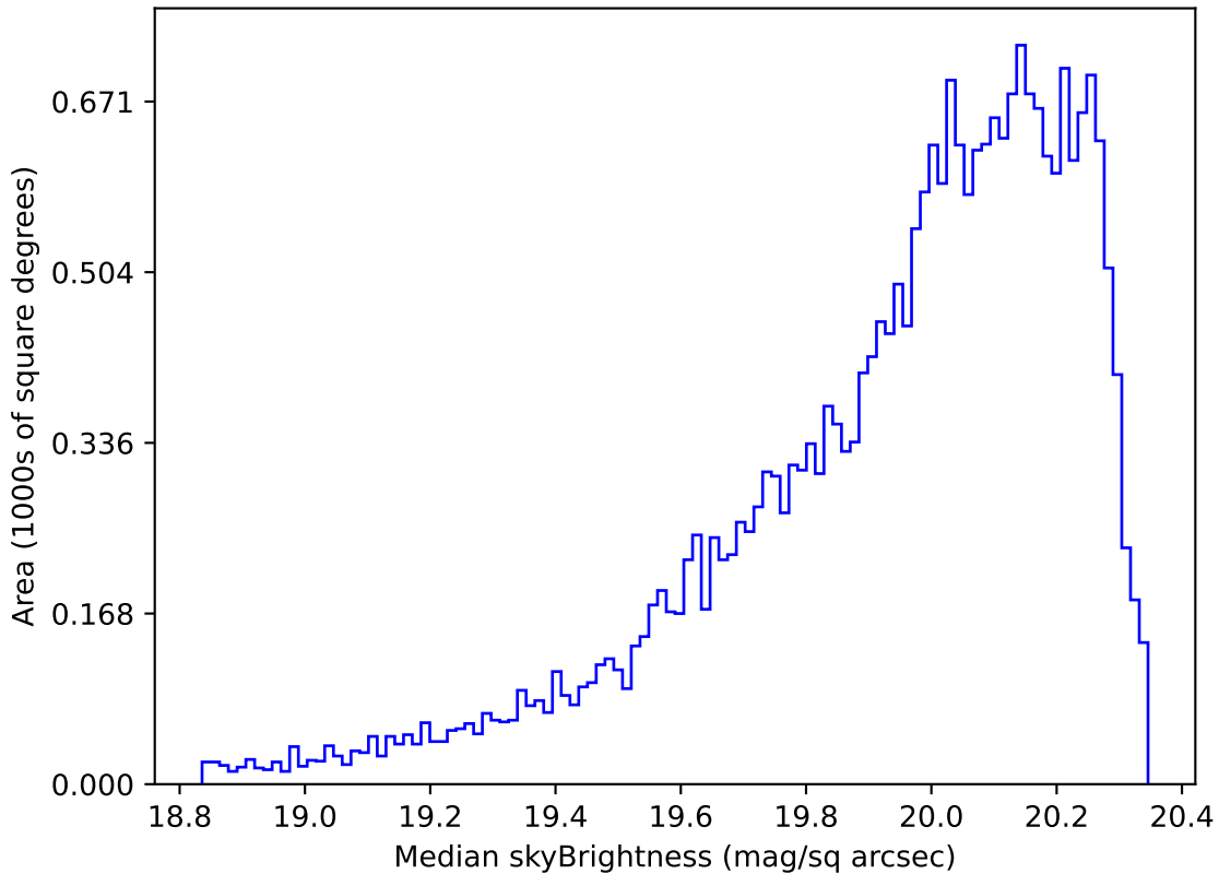
too_elab_r64_d3_ugrizy_v3.4_10yrs Yr 1 i band: Median skyBrightness
