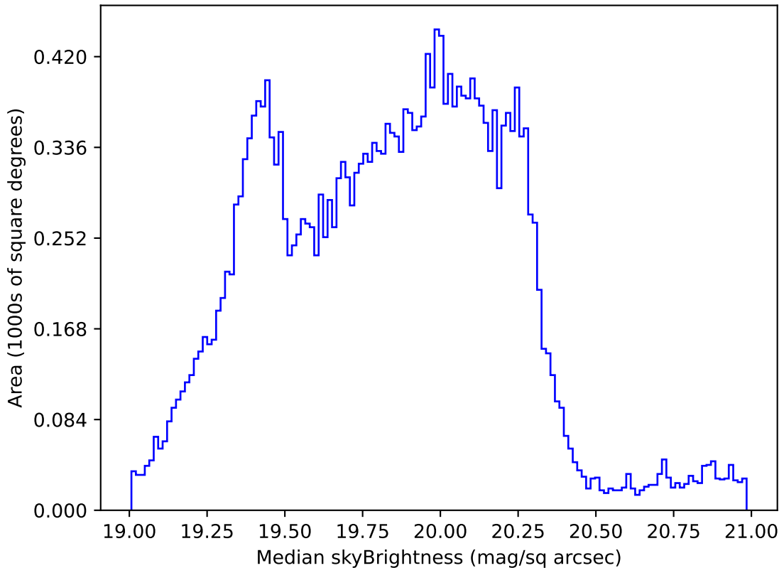
too_elab_r64_d3_ugrizy_v3.4_10yrs Yr 1 all bands: Median skyBrightness
