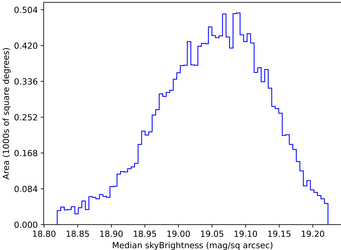
too_elab_r64_d3_ugrizy_v3.4_10yrs WFD z band: Median skyBrightness
