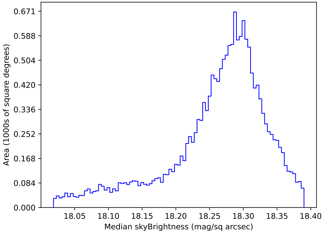
too_elab_r64_d3_ugrizy_v3.4_10yrs WFD y band: Median skyBrightness
