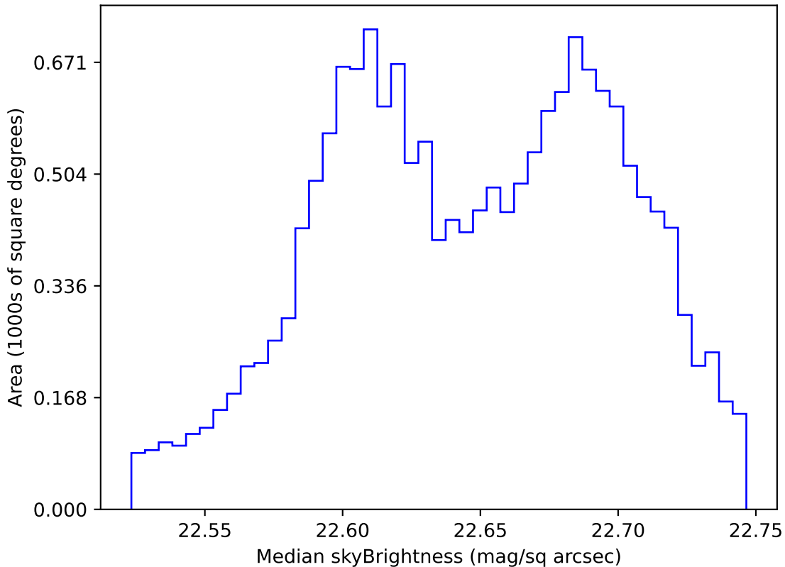
too_elab_r64_d3_ugrizy_v3.4_10yrs WFD u band: Median skyBrightness
