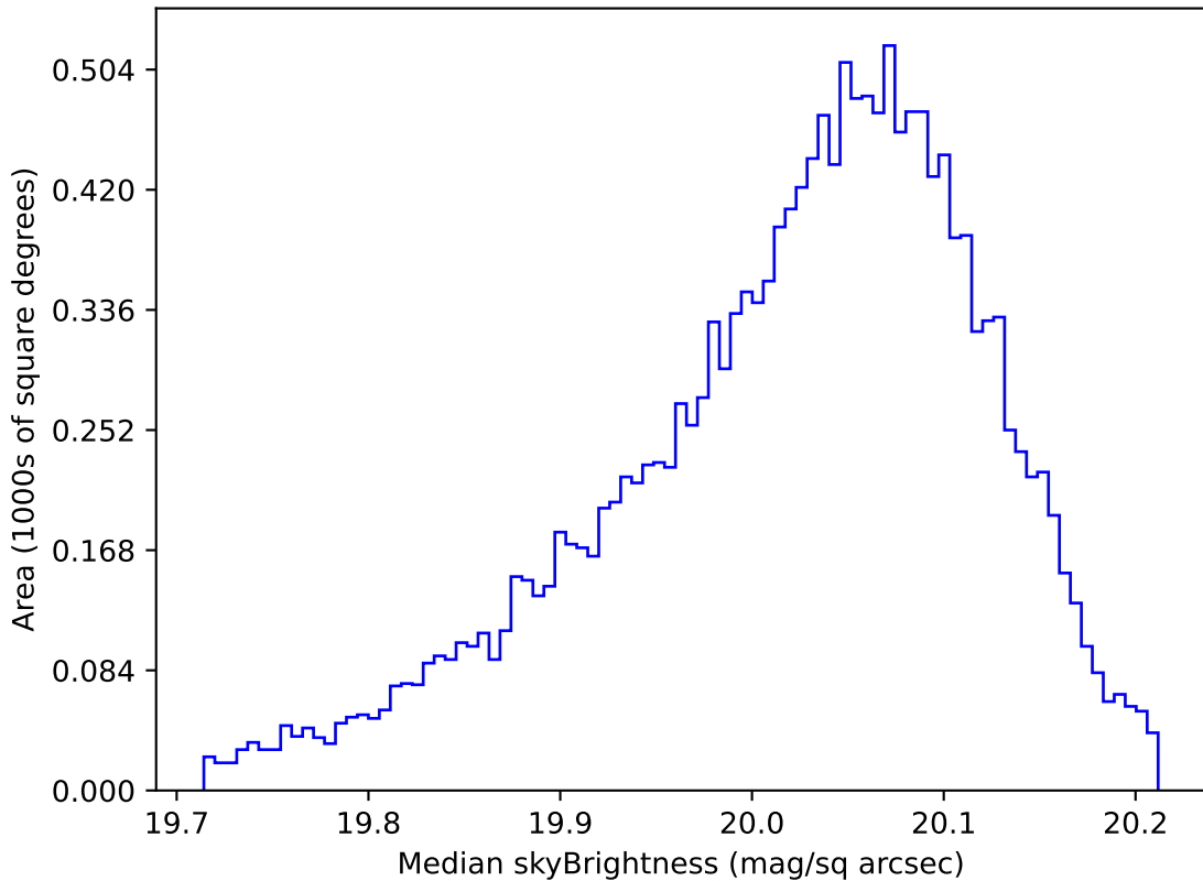
too_elab_r64_d3_ugrizy_v3.4_10yrs WFD i band: Median skyBrightness
