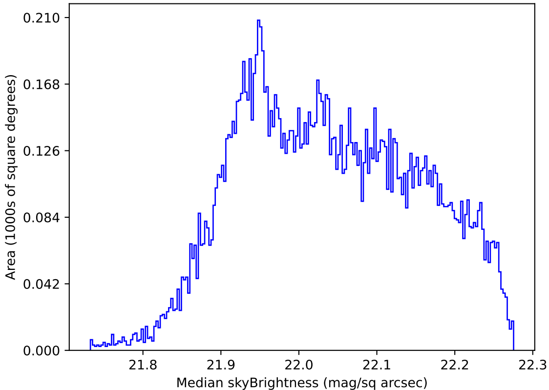
too_elab_r64_d3_ugrizy_v3.4_10yrs WFD g band: Median skyBrightness
