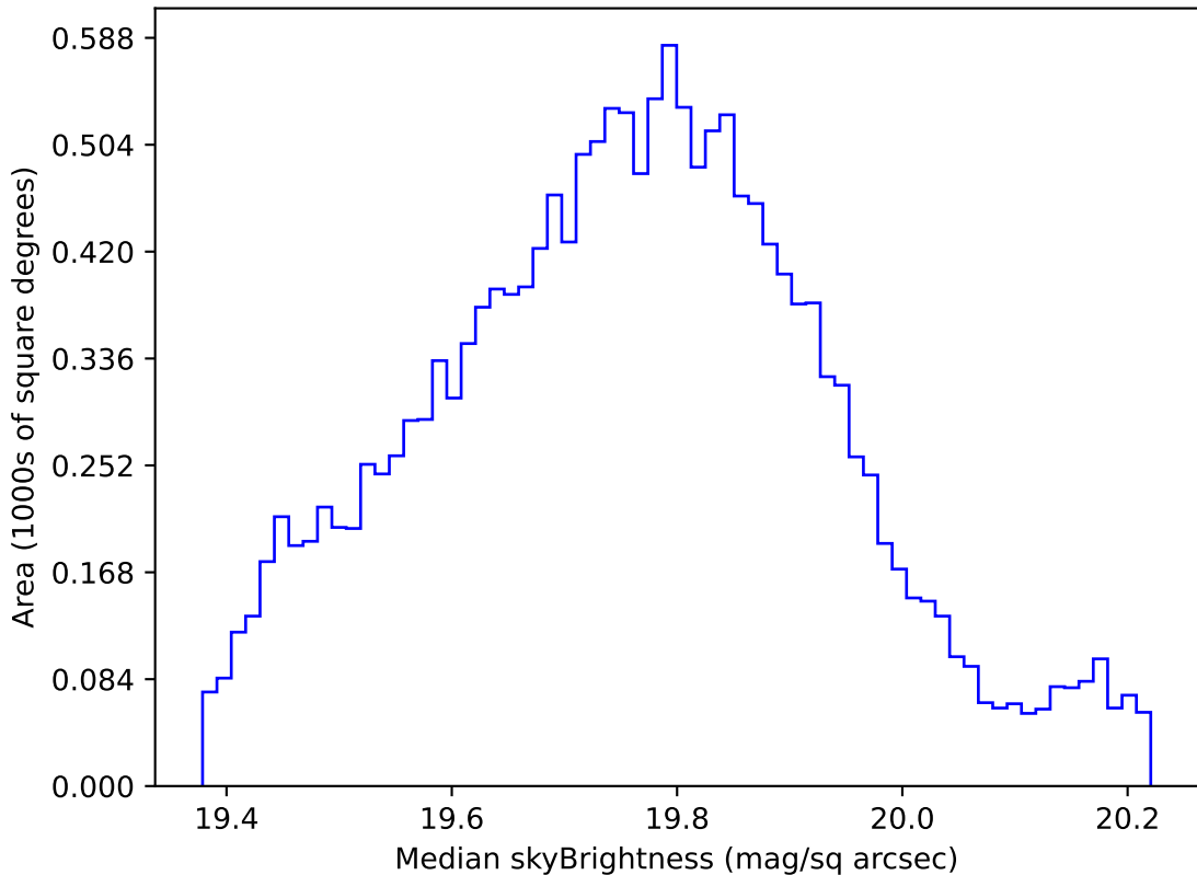
too_elab_r64_d3_ugrizy_v3.4_10yrs WFD all bands: Median skyBrightness
