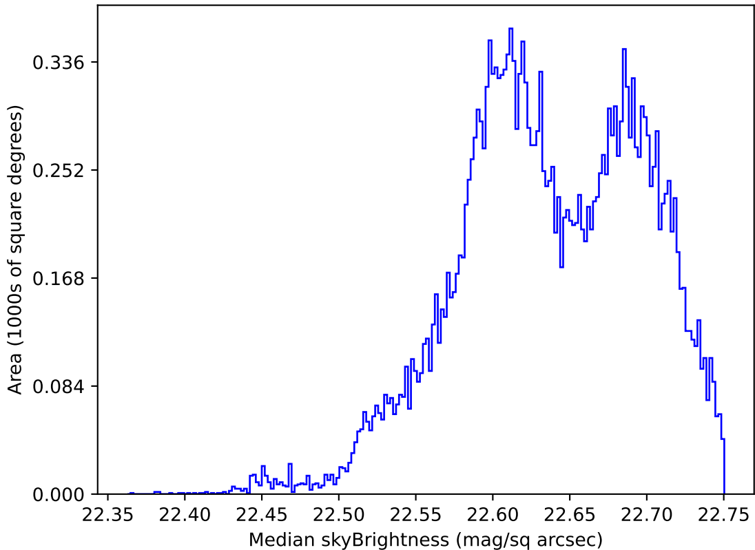
too_elab_r64_d3_ugrizy_v3.4_10yrs All sky u band: Median skyBrightness
