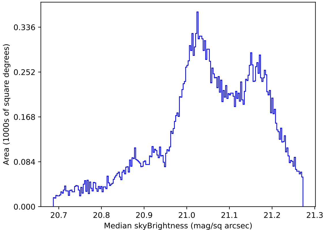
too_elab_r64_d3_ugrizy_v3.4_10yrs All sky r band: Median skyBrightness
