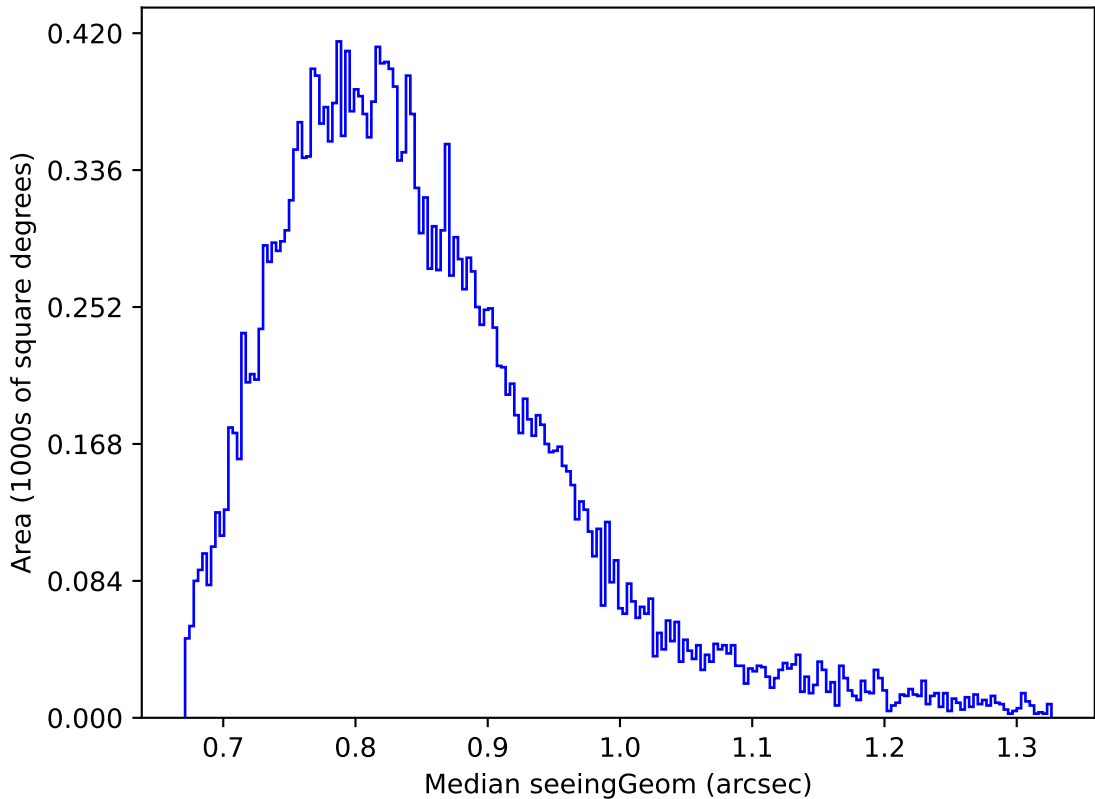
too_elab_r64_d3_ugrizy_v3.4_10yrs Yr 1 z band: Median seeingGeom
