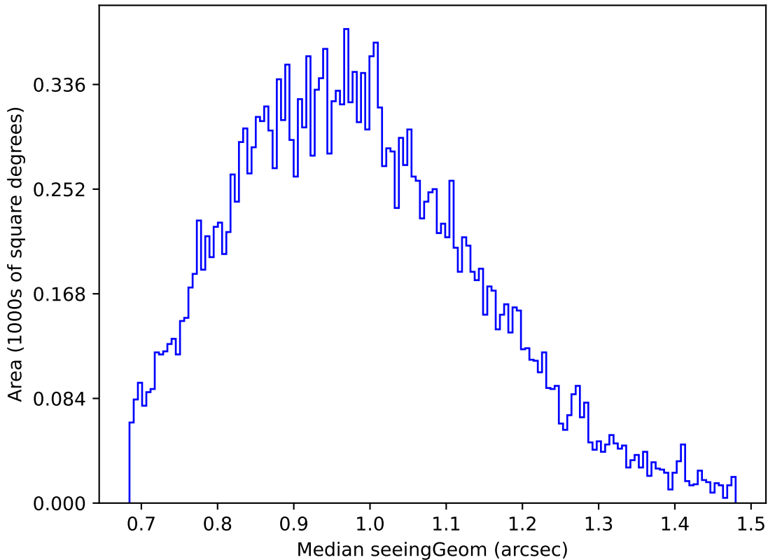
too_elab_r64_d3_ugrizy_v3.4_10yrs Yr 1 u band: Median seeingGeom
