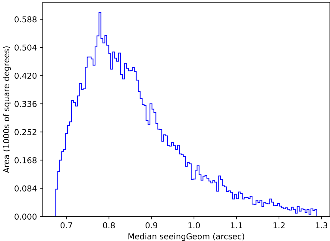
too_elab_r64_d3_ugrizy_v3.4_10yrs Yr 1 r band: Median seeingGeom
