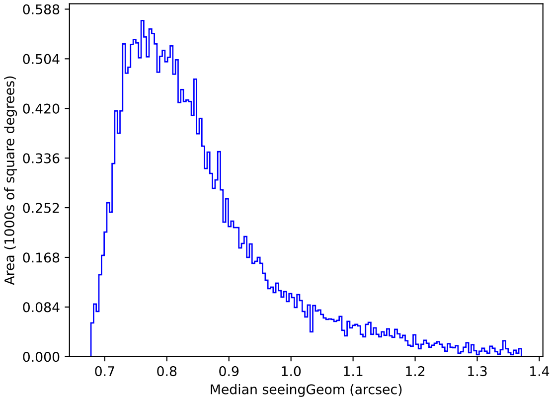
too_elab_r64_d3_ugrizy_v3.4_10yrs Yr 1 i band: Median seeingGeom
