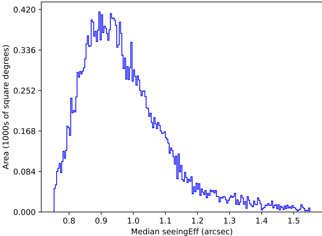
too_elab_r64_d3_ugrizy_v3.4_10yrs Yr 1 z band: Median seeingEff
