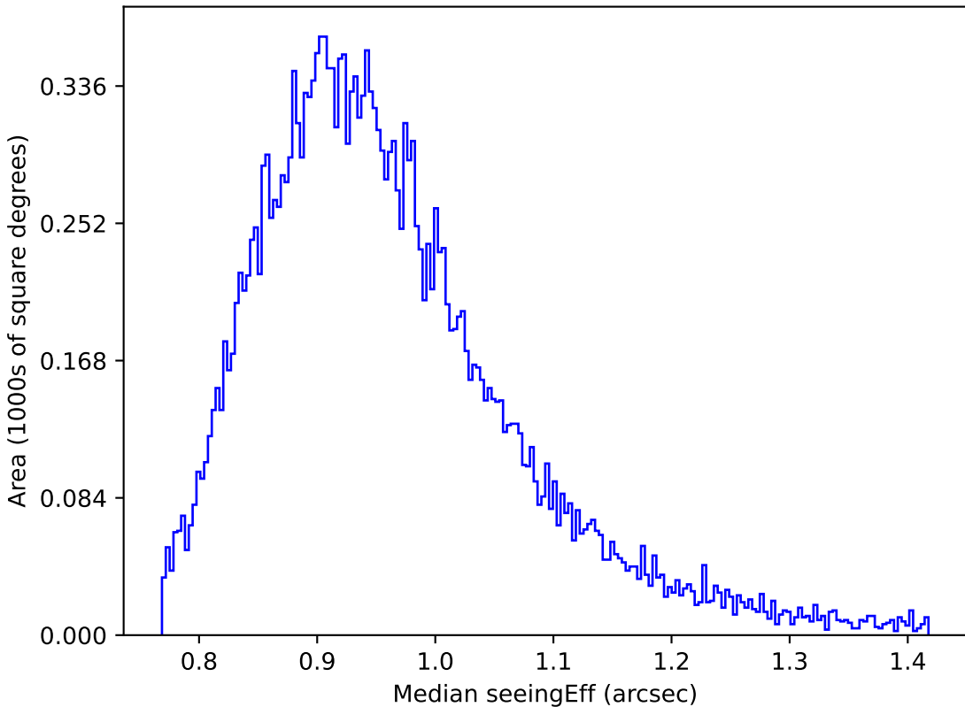
too_elab_r64_d3_ugrizy_v3.4_10yrs Yr 1 y band: Median seeingEff
