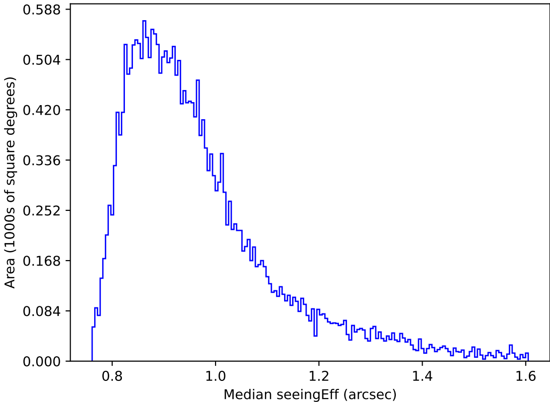
too_elab_r64_d3_uigrizy_v3.4_10yrs Yr 1 i band: Median seeingEff
