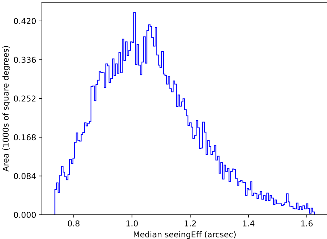
too_elab_r64_d3_ugrizy_v3.4_10yrs Yr 1 g band: Median seeingEff
