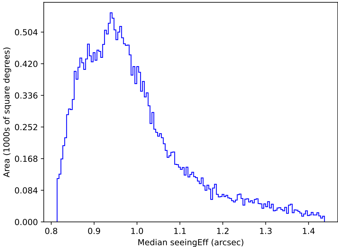
too_elab_r64_d3_ugrizy_v3.4_10yrs Yr 1 all bands: Median seeingEff
