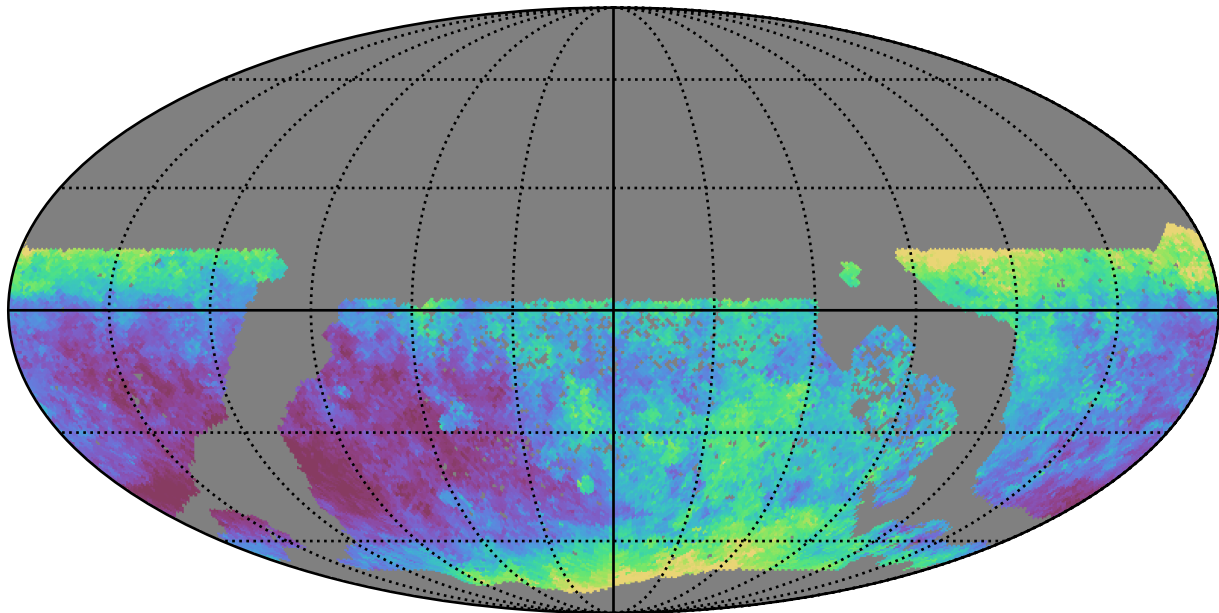
too_elab_r64_d3_ugrizy_v3.4_10yrs WFD z band: Median seeingEff
