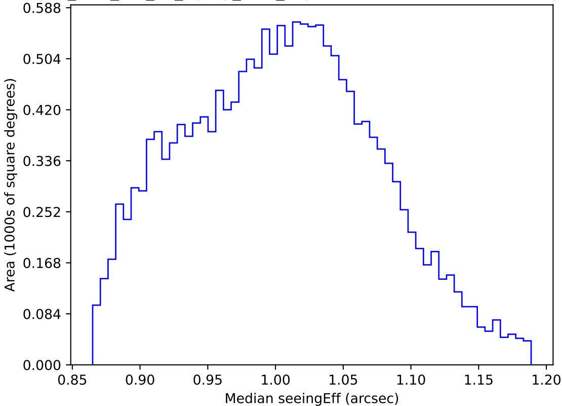
too_elab_r64_d3_ugrizy_v3.4_10yrs WFD z band: Median seeingEff
