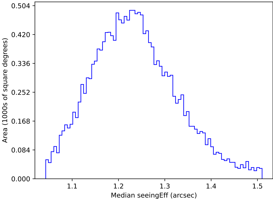
too_elab_r64_d3_ugrizy_v3.4_10yrs WFD u band: Median seeingEff
