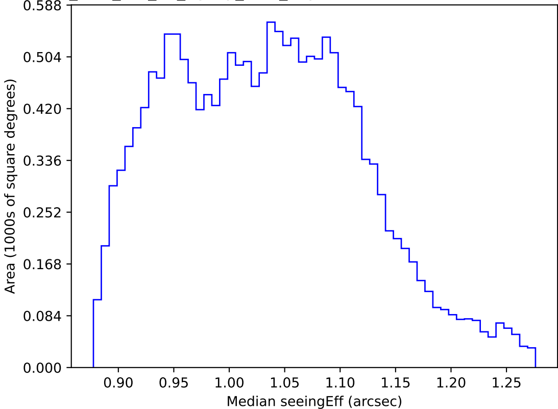
too_elab_r64_d3_ugrizy_v3.4_10yrs WFD r band: Median seeingEff
