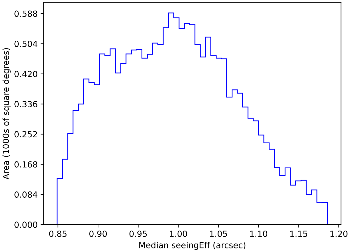
too_elab_r64_d3_ugrizy_v3.4_10yrs WFD i band: Median seeingEff
