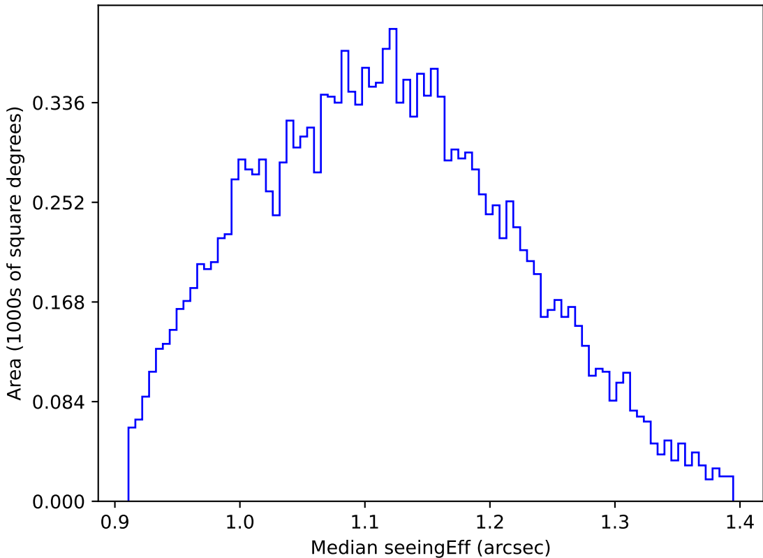
too_elab_r64_d3_ugrizy_v3.4_10yrs WFD g band: Median seeingEff
