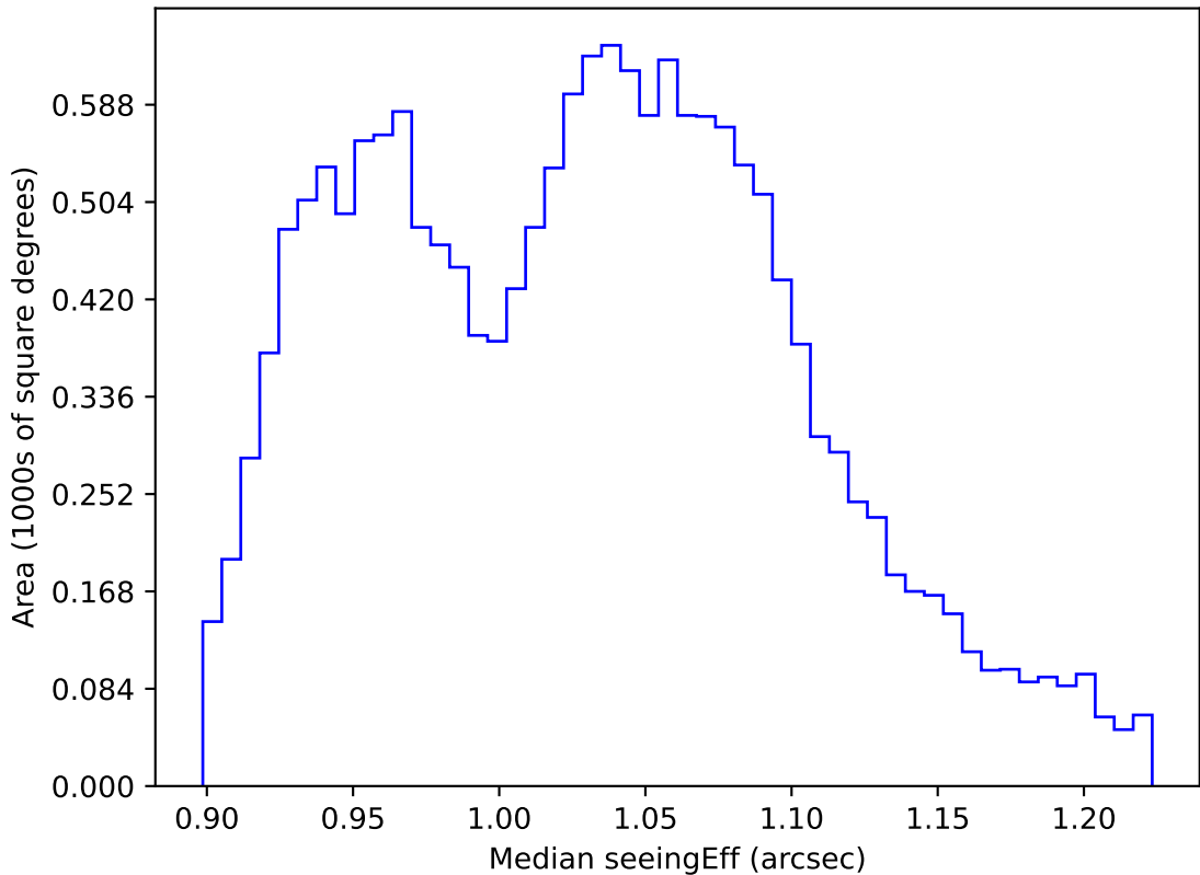
too_elab_r64_d3_ugrizy_v3.4_10yrs WFD all bands: Median seeingEff
