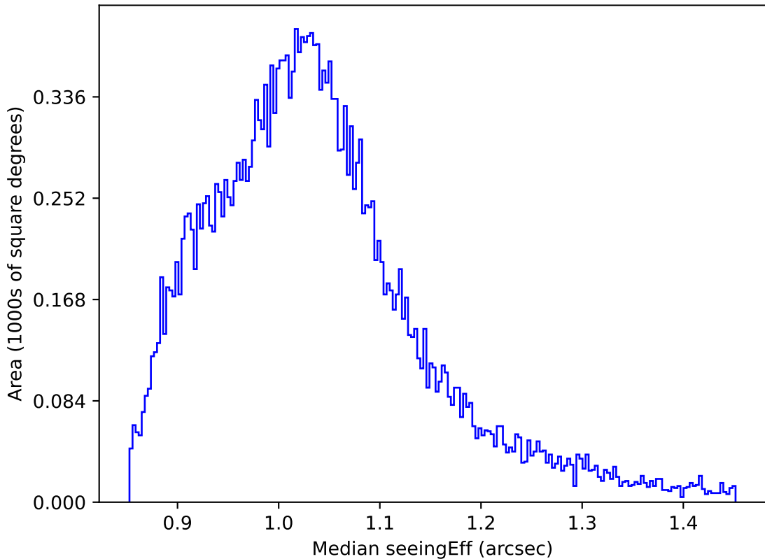
too_elab_r64_d3_ugrizy_v3.4_10yrs All sky z band: Median seeingEff
