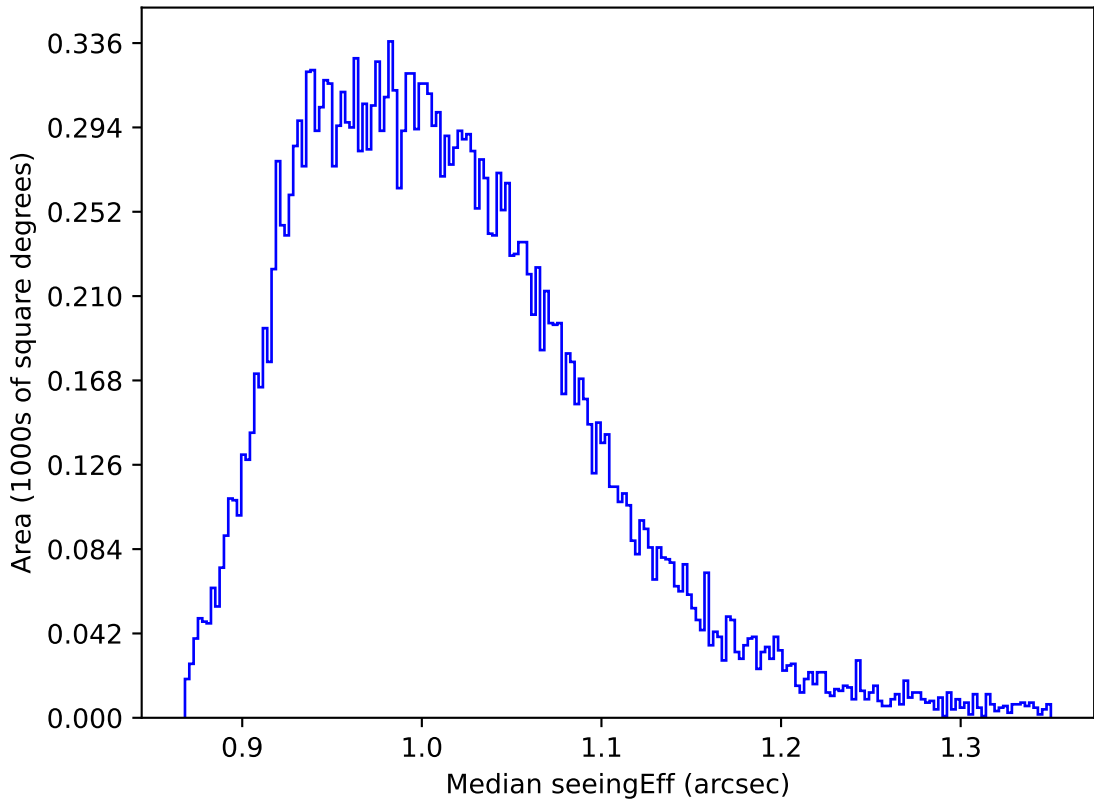
too_elab_r64_d3_ugrizy_v3.4_10yrs All sky y band: Median seeingEff
