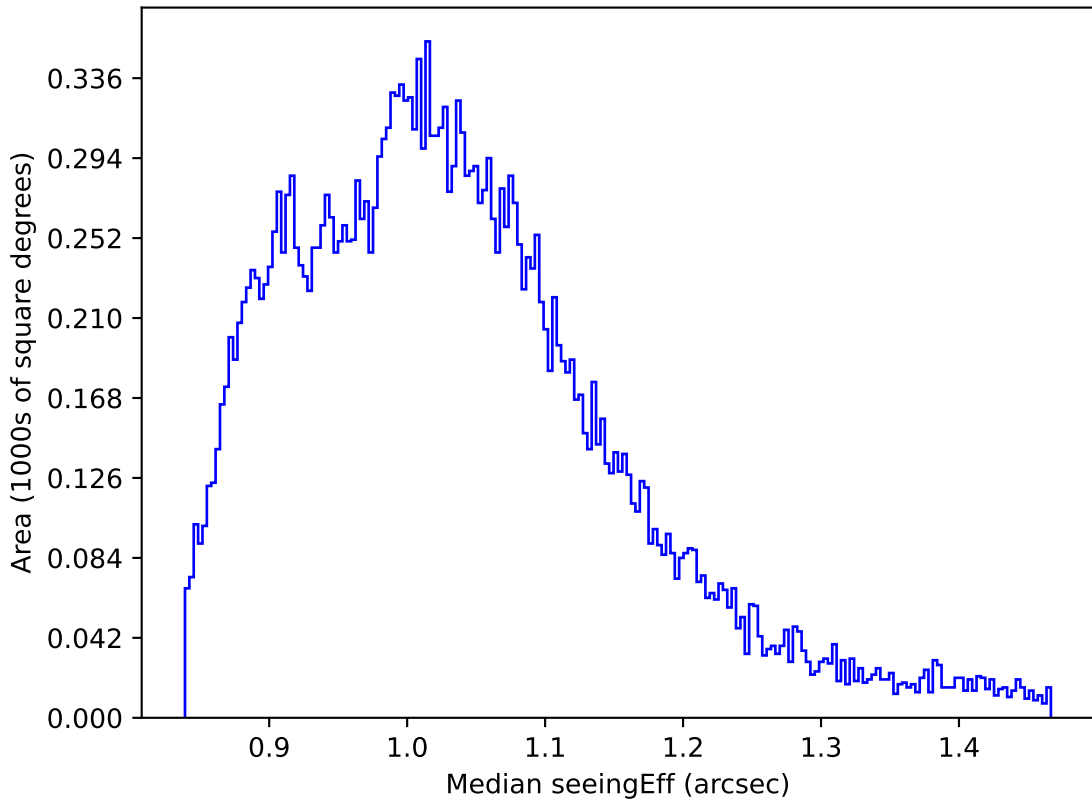
too_elab_r64_d3_ugrizy_v3.4_10yrs All sky i band: Median seeingEff
