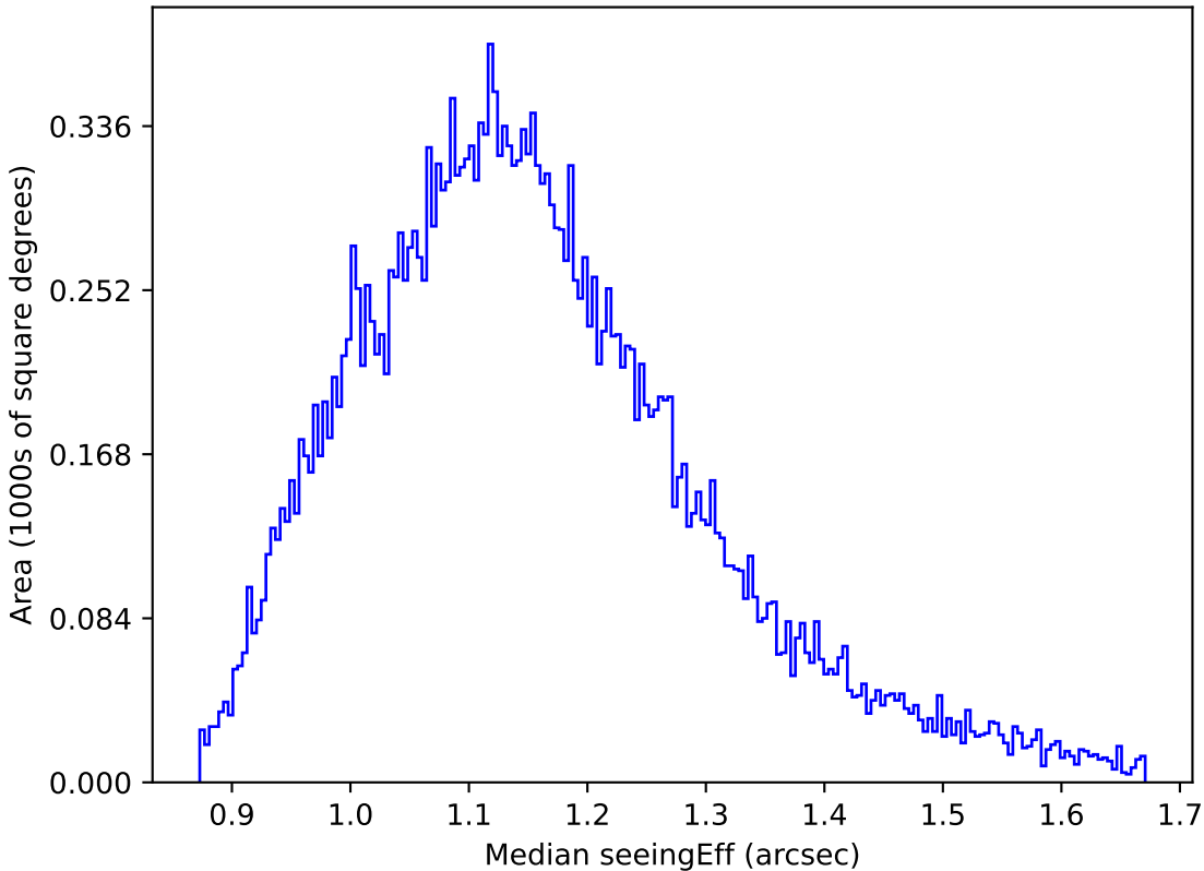
too_elab_r64_d3_ugrizy_v3.4_10yrs All sky g band: Median seeingEff
