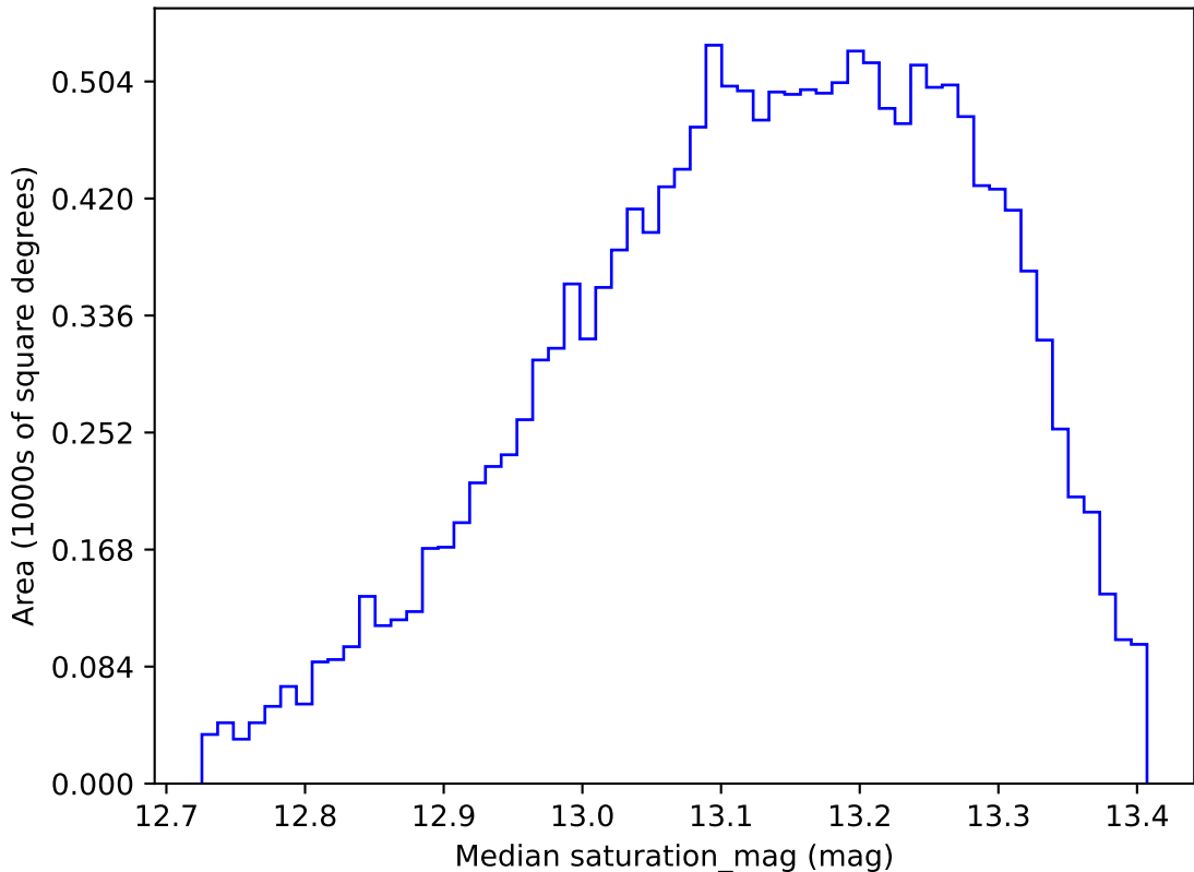
too_elab_r64_d3_ugrizy_v3.4_10yrs WFD y band: Median saturation_mag
