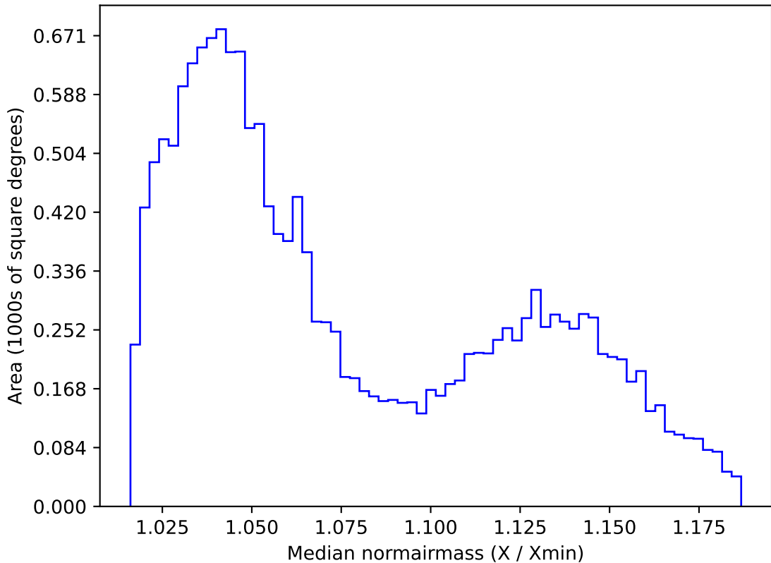
too_elab_r64_d3_ugrizy_v3.4_10yrs WFD r band: Median normairmass
