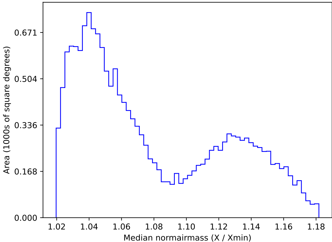
too_elab_r64_d3_ugrizy_v3.4_10yrs WFD i band: Median normairmass
