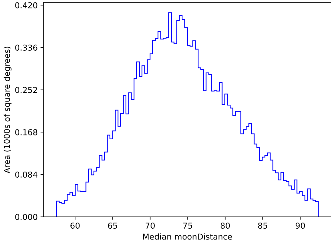
too_elab_r64_d3_ugrizy_v3.4_10yrs WFD z band: Median moonDistance
