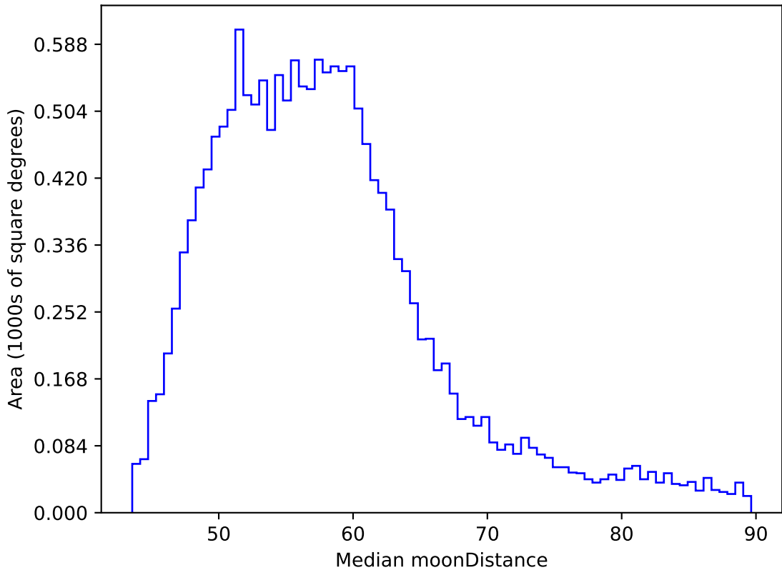
too_elab_r64_d3_ugrizy_v3.4_10yrs WFD y band: Median moonDistance
