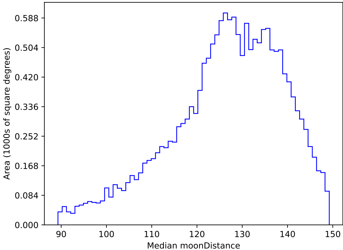
too_elab_r64_d3_ugrizy_v3.4_10yrs WFD u band: Median moonDistance
