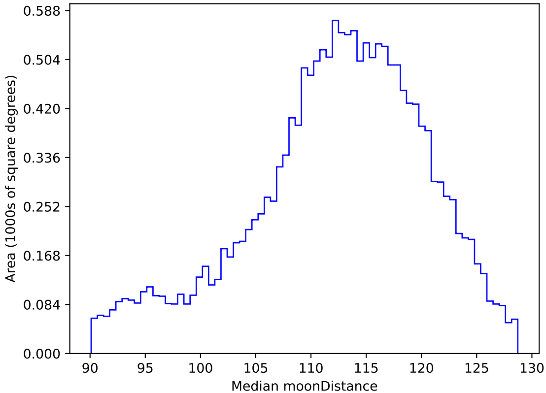
too_elab_r64_d3_ugrizy_v3.4_10yrs WFD r band: Median moonDistance
