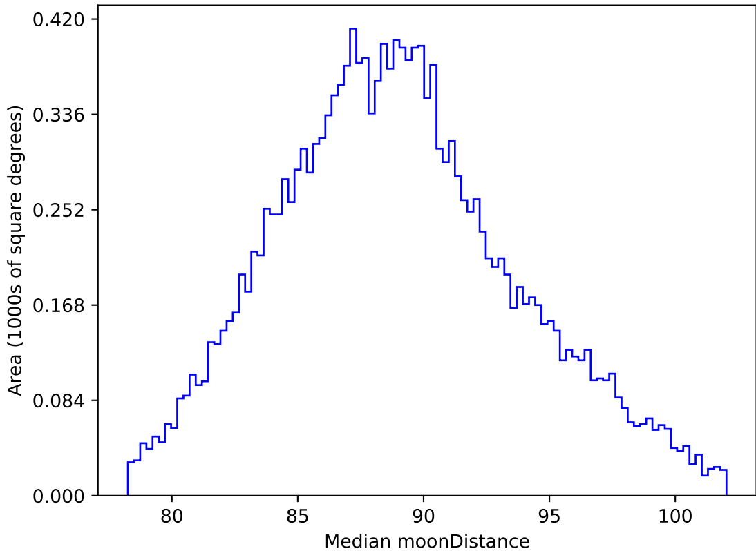
too_elab_r64_d3_ugrizy_v3.4_10yrs WFD all bands: Median moonDistance
