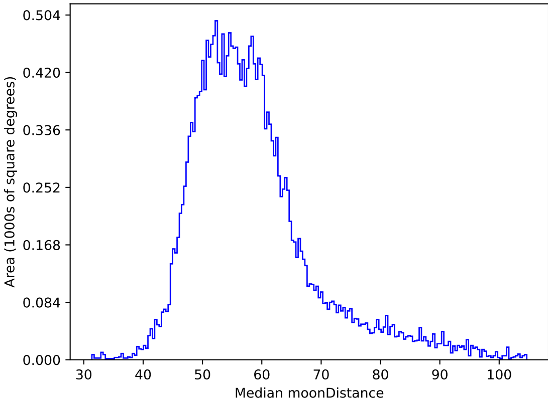
too_elab_r64_d3_ugrizy_v3.4_10yrs All sky y band: Median moonDistance
