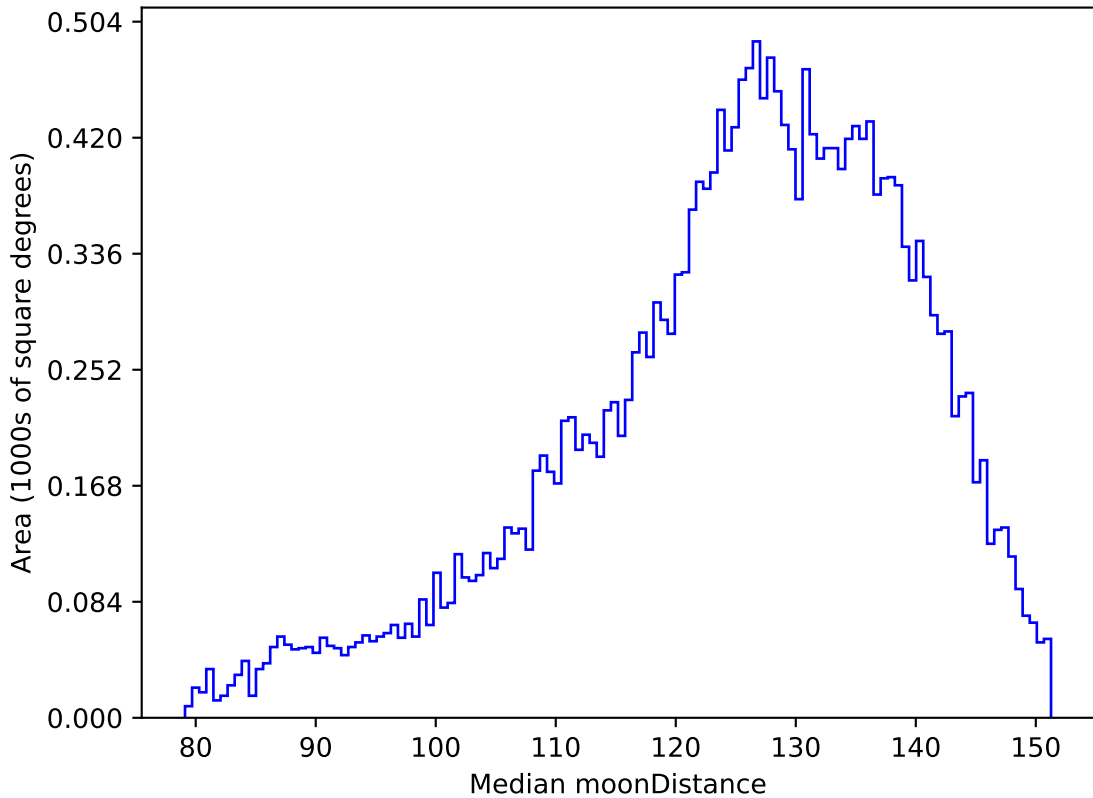
too_elab_r64_d3_ugrizy_v3.4_10yrs All sky u band: Median moonDistance
