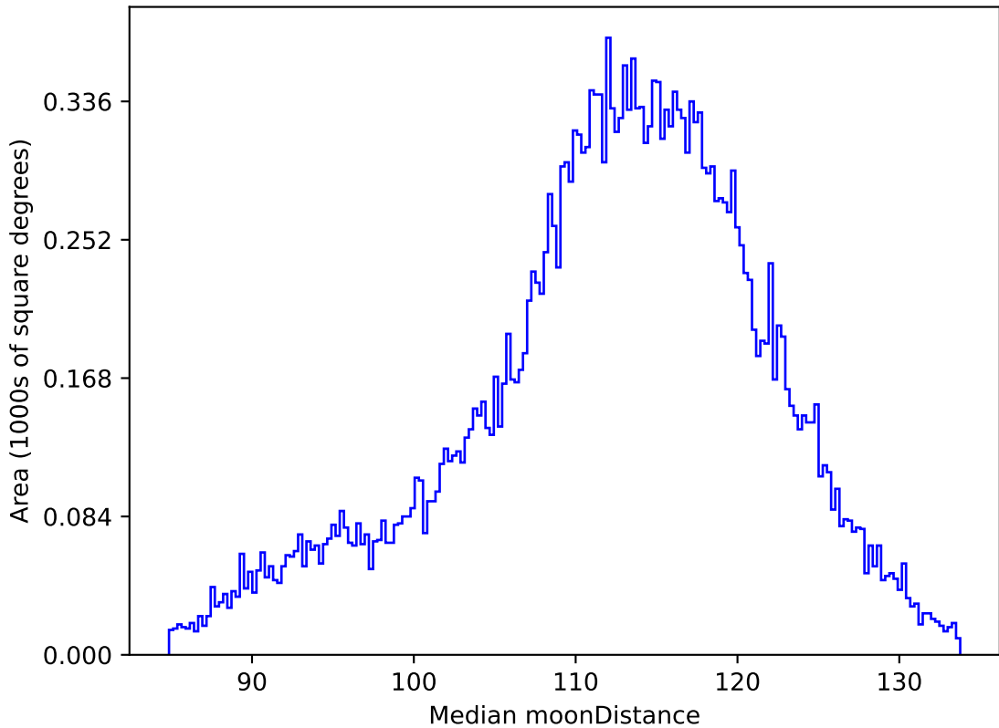
too_elab_r64_d3_ugrizy_v3.4_10yrs All sky r band: Median moonDistance
