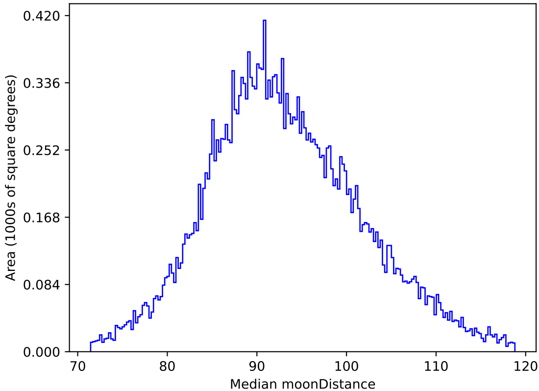
too_elab_r64_d3_ugrizy_v3.4_10yrs All sky i band: Median moonDistance
