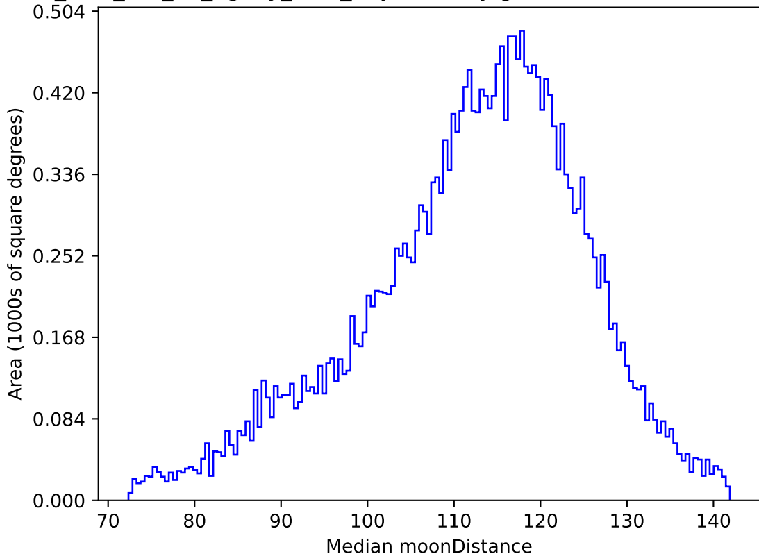
too_elab_r64_d3_ugrizy_v3.4_10yrs All sky g band: Median moonDistance
