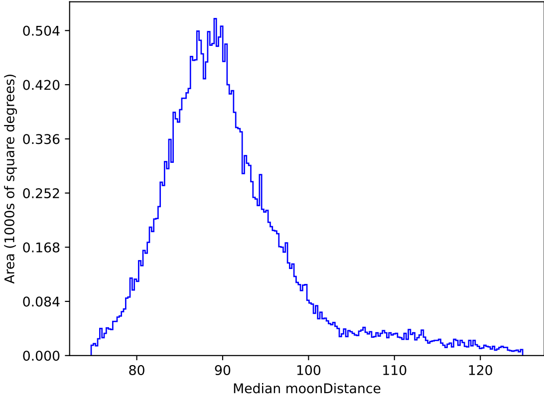
too_elab_r64_d3_ugrizy_v3.4_10yrs All sky all bands: Median moonDistance
