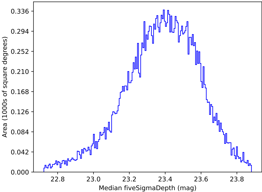
too_elab_r64_d3_ugrizy_v3.4_10yrs Yr 1 all bands: Median fiveSigmaDepth
