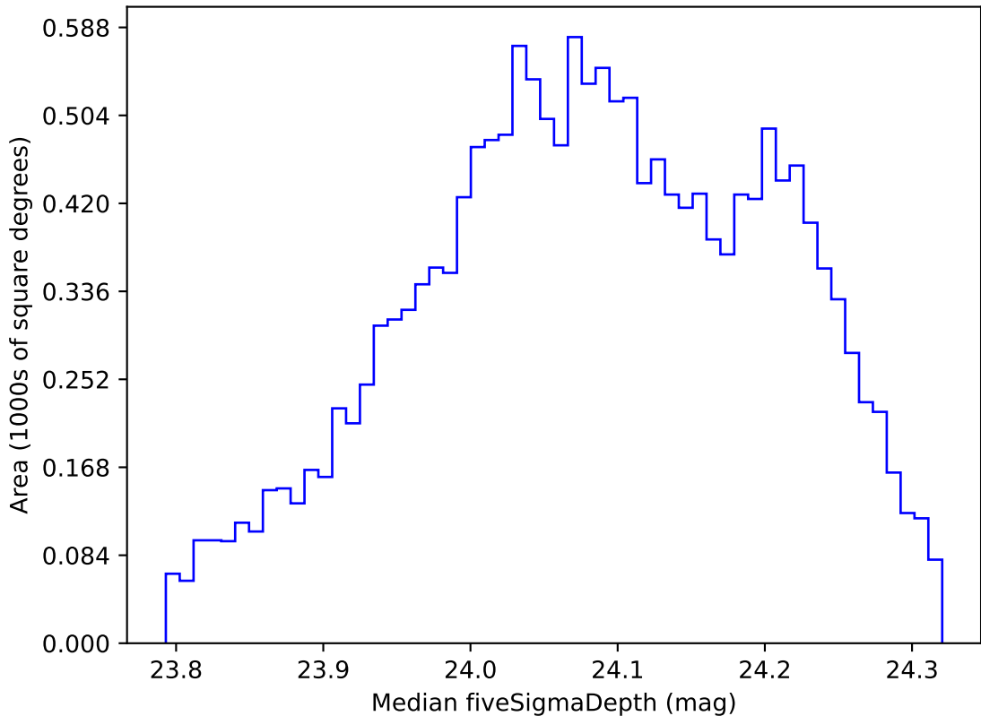
too_elab_r64_d3_ugrizy_v3.4_10yrs WFD r band: Median fiveSigmaDepth
