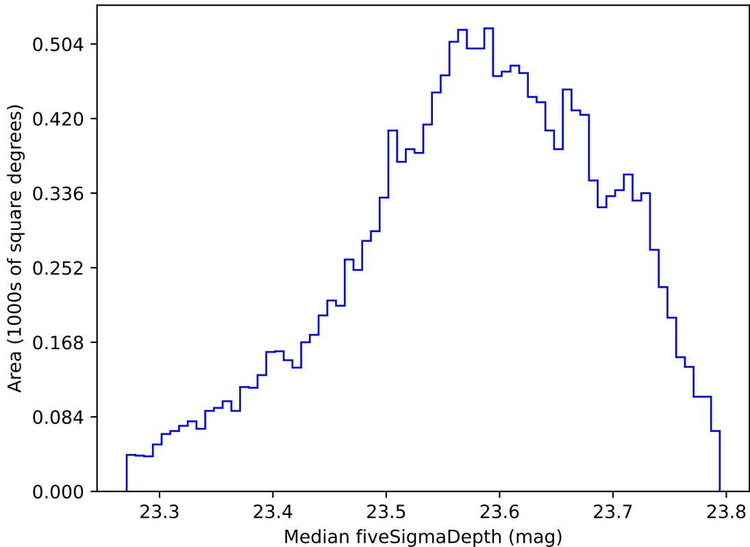
too_elab_r64_d3_ugrizy_v3.4_10yrs WFD i band: Median fiveSigmaDepth
